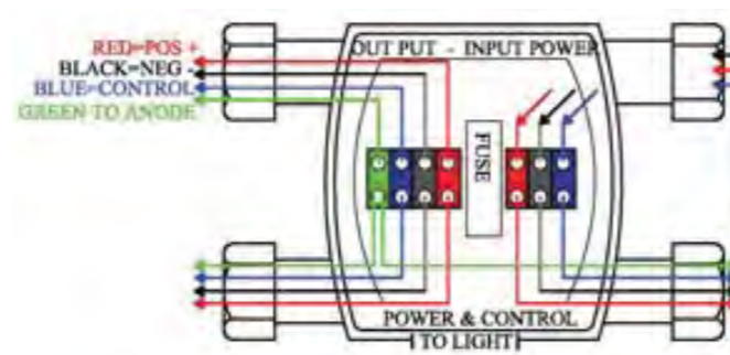
TWO WAY FUSED ENCLOSURE FROM EITHER SIDE - EARTH CONNECTED TO ANODE
