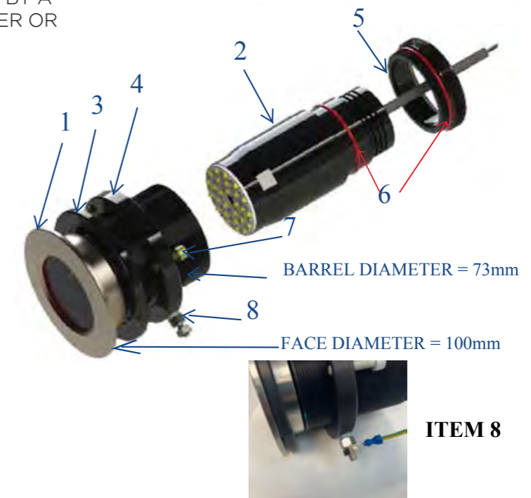
EARTH SCREW
